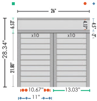
FLAT-DIRM501
