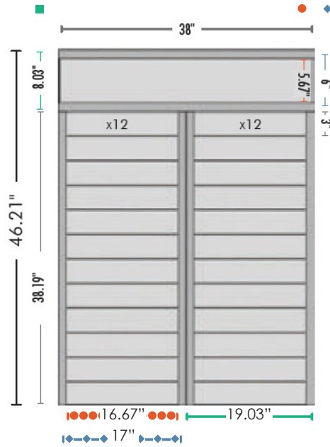
FLAT-DIRM502
